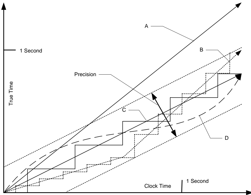
Figure 1: Time base precision in a T&M system
